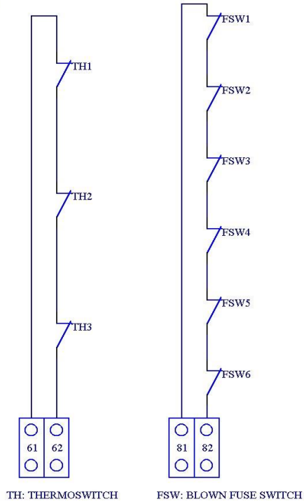
TH: THERMOSWITCH
